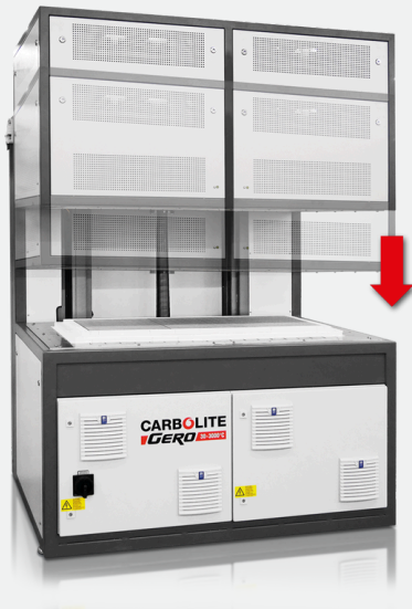
HB 13/240 with optional preheated hot air blowers
